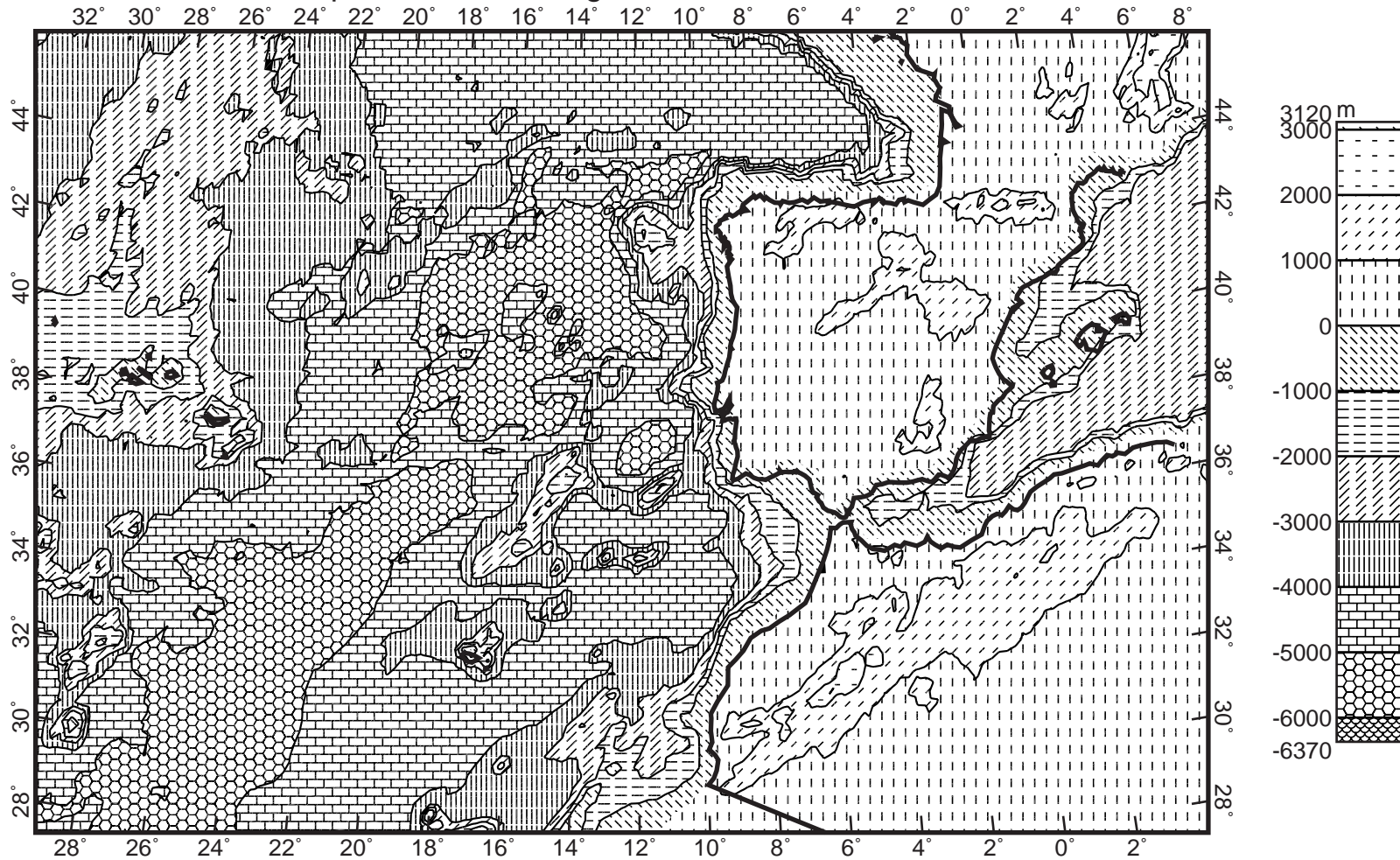
Topography of the Iberian margin plotted from data gridded at 15' intervals
